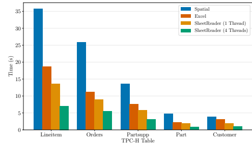
Figure 4: DuckDB spreadsheet loading runtime on TPC-H tables: core extensions (Excel, Spatial) vs. SheetReader.
